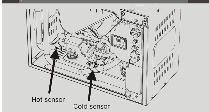
Temperature sensor location
